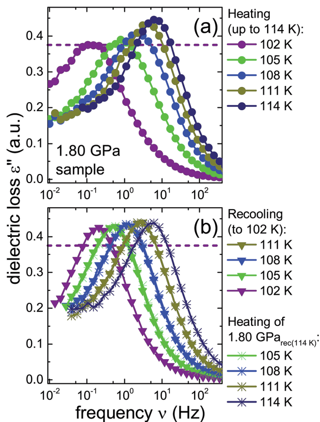
Fig. 6 Dielectric loss spectra of the same 1.80 GPa sample (ice β-XV) for which data are shown in Fig. 4. (a) Spectra measured upon first heating to 114 K are re-plotted here with a zoomed frequency scale to facilitate comparison with subsequent measurements on this sample. (b) Triangles represent data obtained during subsequent cooling which yielded sample 1.80 GPa rec(114 K) . The spectra recorded upon heating of this sample are represented in (b) as asterisks. The dashed lines refer to the amplitude of the dielectric loss spectrum measured at 102 K for the 1.80 GPa sample upon first heating. To guide the eye, data points are connected by lines.
